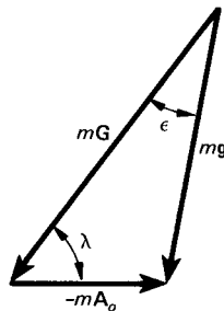
FIGURE 4.10 Vector diagram defining the quantity m\mathbf{g} .
