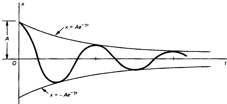
FIGURE 2.9 Graph of displacement versus time for the underdamped harmonic oscillator.
