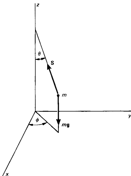
FIGURE 3.11 The spherical pendulum.
