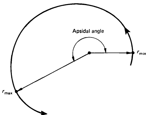
FIGURE 5.10 The apsidal angle.
