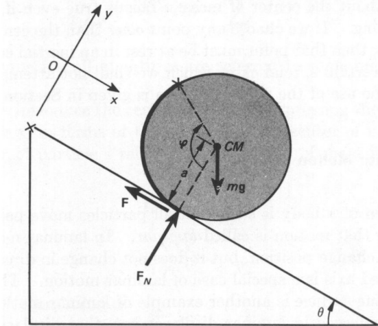
FIGURE 7.11 Body rolling an inclined plane.
