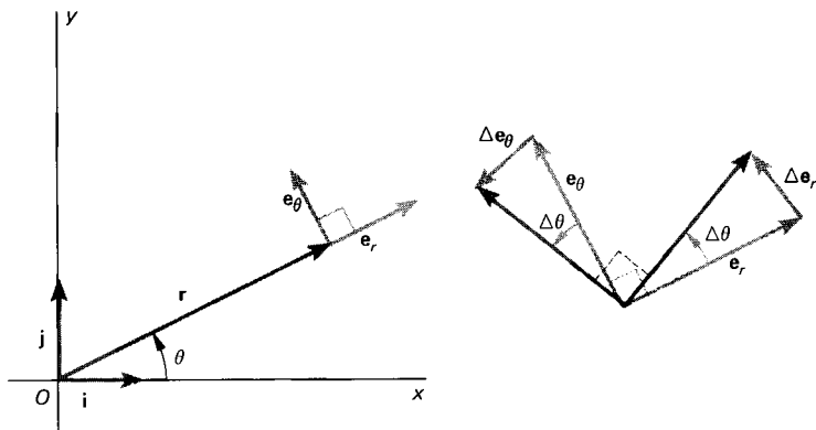
FIGURE 1.19 Unit vectors for plane polar coordinates.
