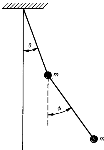
FIGURE 10.5 The double pendulum.
