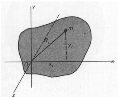
FIGURE 7.7 The perpendicular axis theorem.
