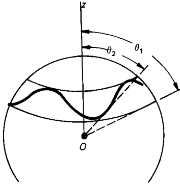
FIGURE 8.18 Illustrating the nutation of a simple gyroscope.
