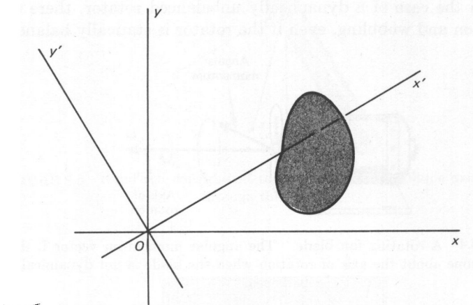
FIGURE 8.3 Rotated axes.
