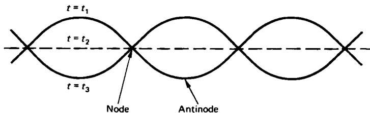
FIGURE 10.11 Standing waves.
